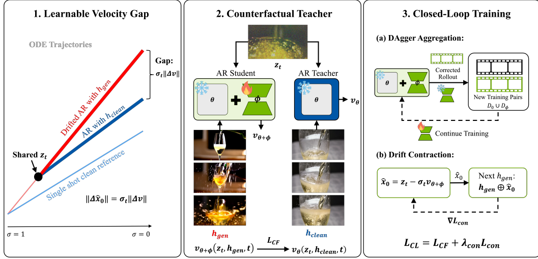
Figure 2: Overview of Clean Forcing. (1) At the shared noisy state z_t , \Delta v := v_{\theta}(z_t, h_{\text{clean}}, t) - v_{\theta}(z_t, h_{\text{gen}}, t) is the history-induced velocity gap. The corresponding one-step clean-latent predictions differ by \sigma_t \|\Delta v\| , contributing to drift over successive chunks. (2) The LoRA student conditions on h_{\text{gen}} and matches the frozen teacher’s prediction under h_{\text{clean}} ( \mathcal{L}_{\text{CF}} ) ( \phi denotes the weights of the LoRA corrector r_{\phi} ). (3a) We generate new training pairs D_{\phi} with the corrector active and continue training on D_0 \cup D_{\phi} , where D_0 contains pairs from uncorrected rollouts. (3b) \mathcal{L}_{\text{con}} backpropagates the next chunk’s error through the undetached prediction \hat{x}_0 .
