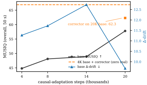
Figure 6: Longer causal adaptation does not replace correction. MUSIQ (black, left axis) improves from 4K to 20K steps, but \Delta -drift (blue, right axis) remains substantial. The corrected 4K base reaches 66.9 MUSIQ (dashed line); a corrector retrained on the 20K base reaches 62.3 (square).
