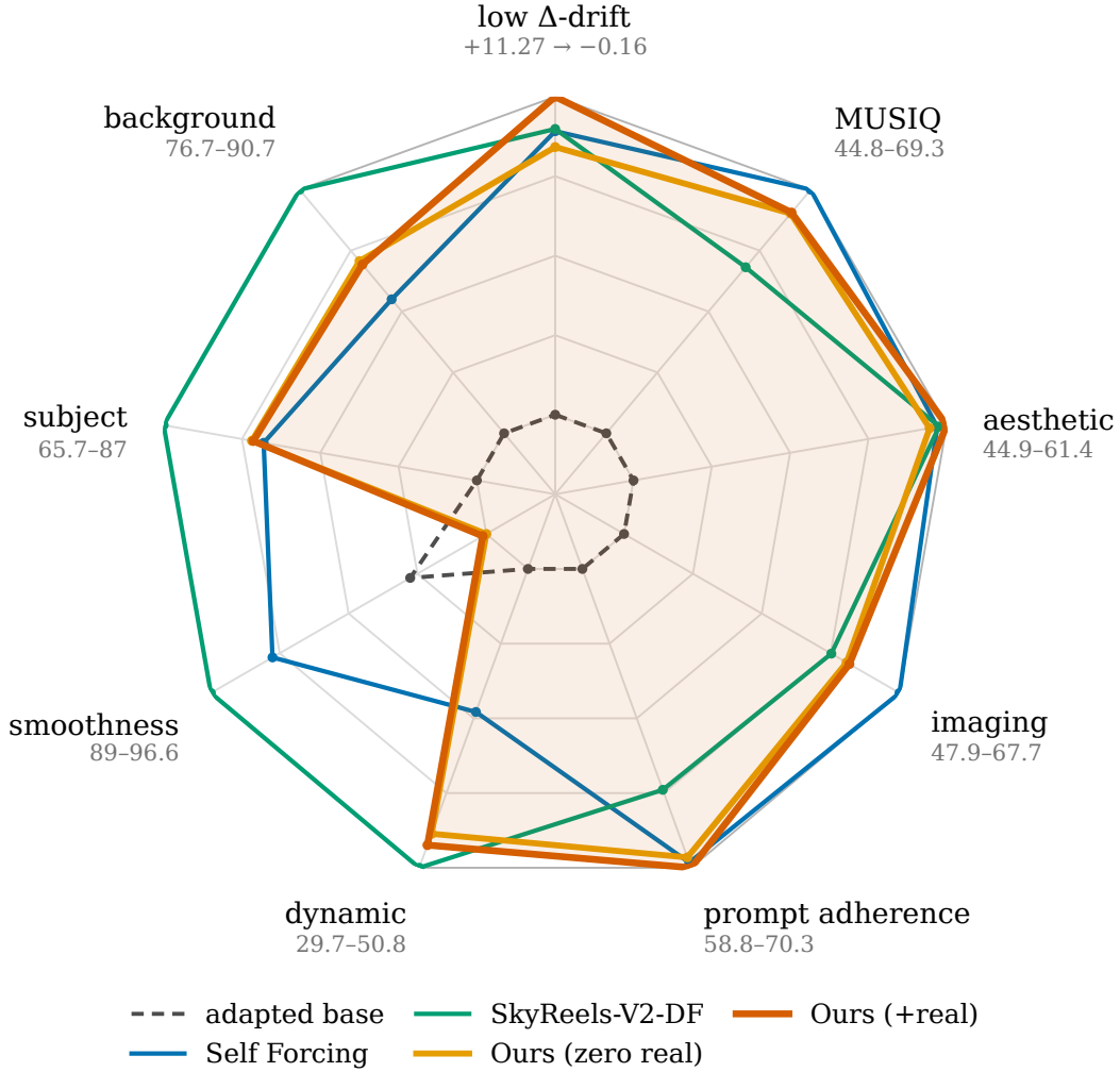
Figure 12: VBench and drift comparison. Scores from Tables 1 and 13 are normalized by axis; the drift axis is reversed so that outward is better. Clean Forcing improves the adapted base across most measures and is competitive with the retrained models, though it remains lower on smoothness and consistency.
