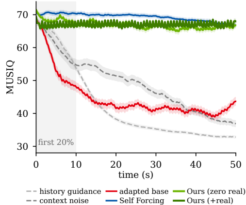
Figure 3: Per-frame quality over 50 s. Mean MUSIQ \pm SEM across 128 prompts. Both Clean Forcing variants remain stable as the base and training-free baselines decline. Ripples mark chunk boundaries.
