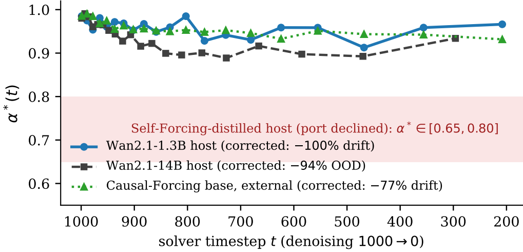
Figure 7: Systematic velocity gap across bases. Per-timestep \alpha^*(t) (Eq. 3) is high on the three bases that benefit from correction (markers). The Self Forcing distilled generator has a lower measured range, [0.65, 0.80] (shaded band), and its corrected rollout deteriorates. All measurements precede corrector training.
