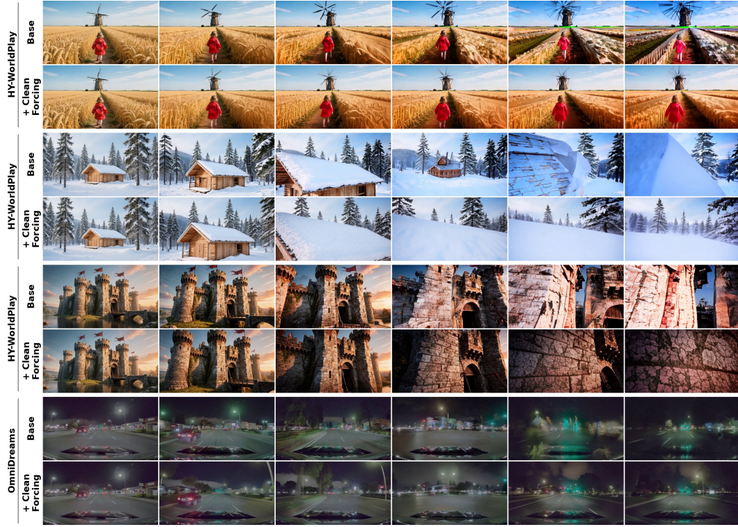
Figure 11: Correction on other autoregressive world models. Six evenly spaced frames from three HY-WorldPlay rollouts ( \sim 24 s) and one OmniDreams driving rollout ( \sim 80 s). Each base and corrected pair shares its prompt, conditioning, and seed. We use strengths of 0.5\alpha^*(t) for HY-WorldPlay and 0.25\alpha^*(t) for OmniDreams. The corrected rollouts better retain color, detail, and scene structure as the base rollouts degrade.
